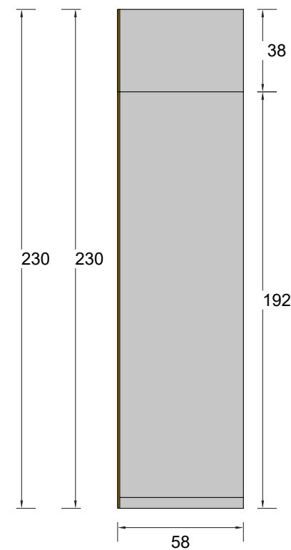
SIDE ELEVATION
