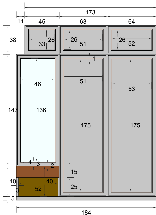
FRONT ELEVATION
